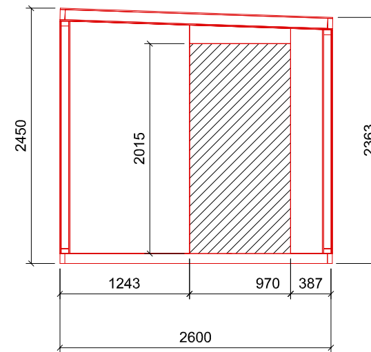
RH Elevation
