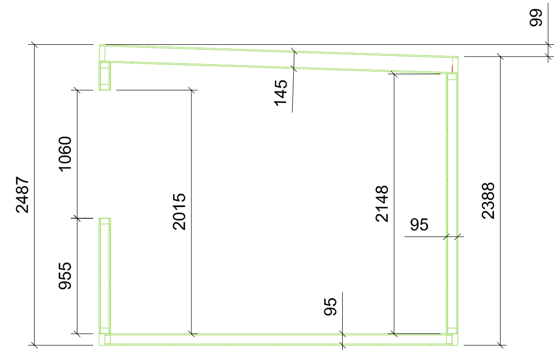
Sections
