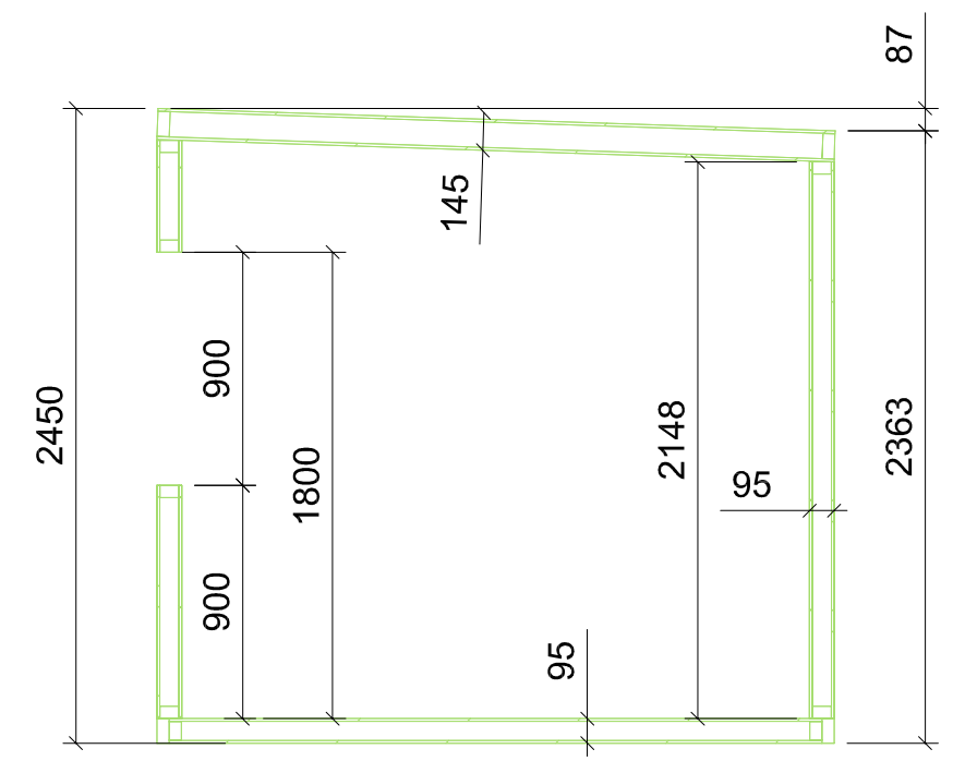
Sections
