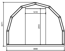
3100mm HIGH POD
